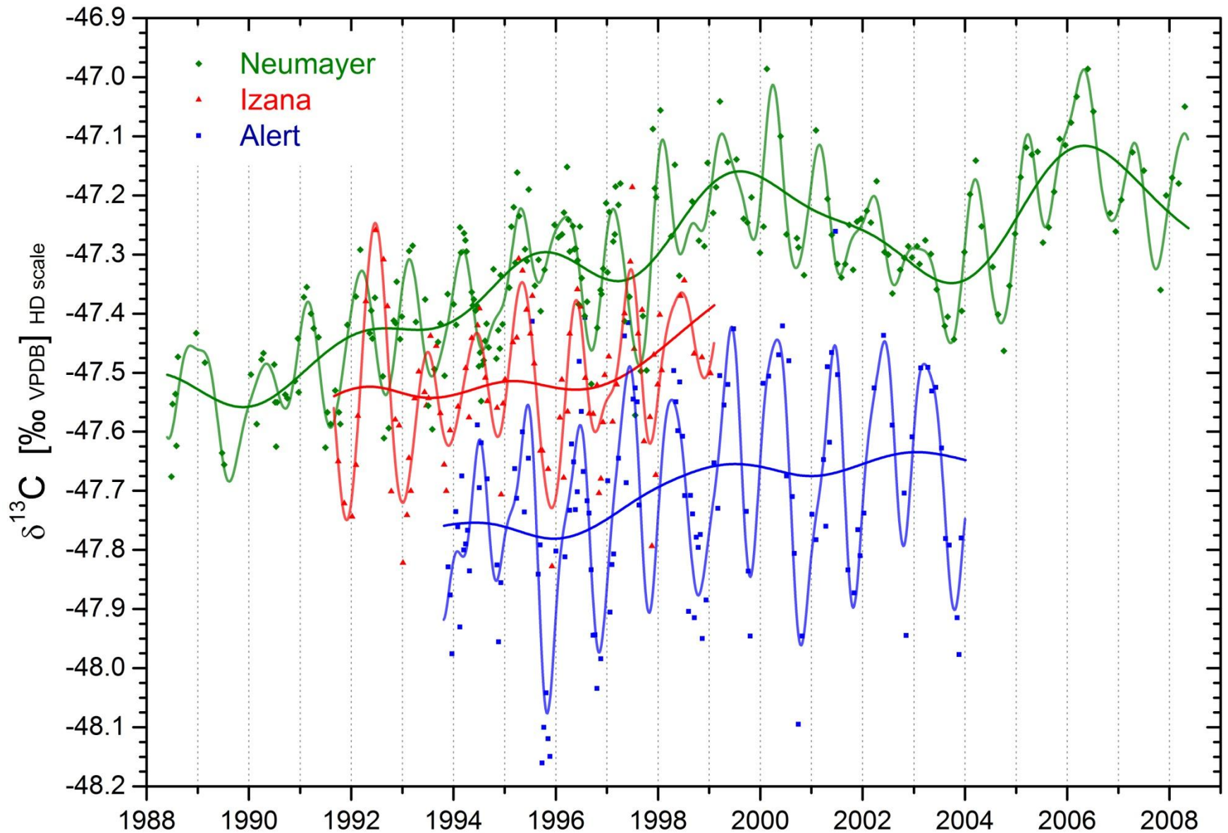
\delta^{13}\text{C}(\text{CH}_4) records of clean air monitoring stations at Alert (Ellesmere Island, Nunavut, Canada) 82.45°N 62.52°W 210m a.s.l., Izaña (Tenerife/Spain) 28.30°N 16.48°W 2367m a.s.l., and Neumayer Station (Dronning Maud Land, Antarctica) 70.65°S 8.25°W 42m a.s.l. \delta^{13}\text{C} values on UHEI scale; Harmonic fits as in Levin I., C. Veidt, B. H. Vaughn, G. Brailsford, T. Bromley, R. Heinz, D. Lowe, J. B. Miller, C. Poß, and J. W. C. White, No inter-hemispheric \text{d}^{13}\text{C}\text{H}_4 trend observed, Nature, Vol.486, 28.6.2012, pages E3-E4, doi:10.1038/nature11175. Neumayer data and fit slightly modified.
